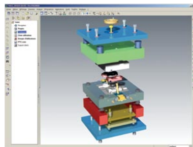
An exploded moldbase in Pro/ENGINEER Expert Moldbase.
